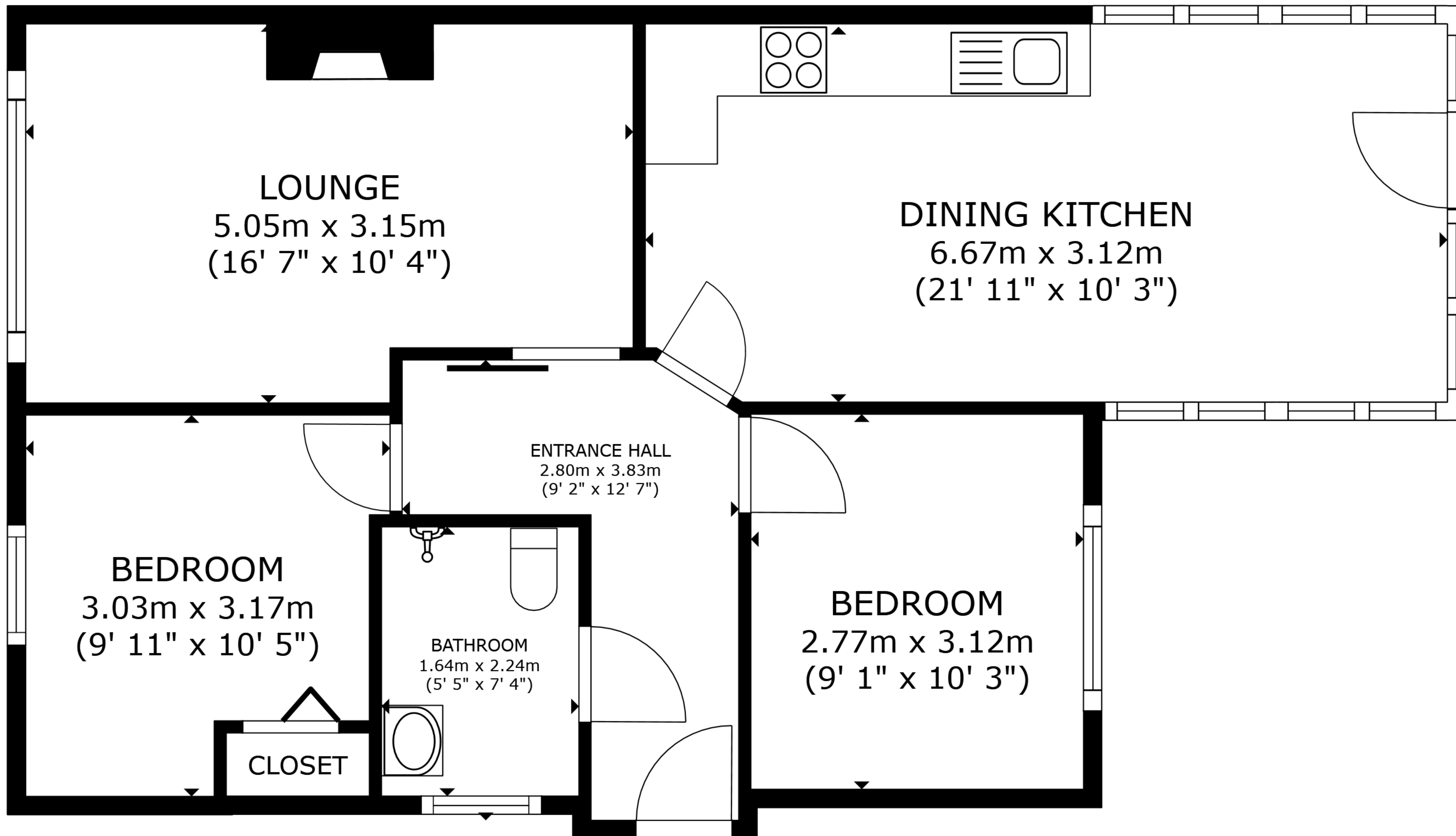
FLOOR PLAN
